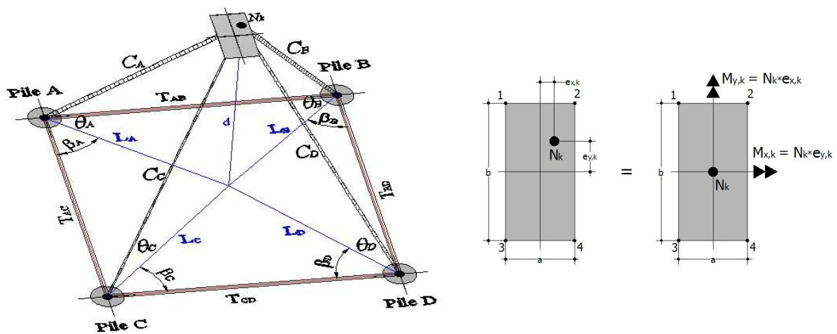
Fig. 1 – Proposed strut-and-tie model for four-pile caps and positive signal convention for biaxial flexure
